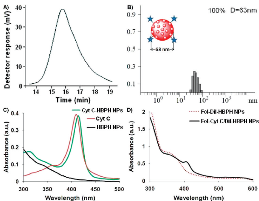
Figure 1. Characterization of the aliphatic HBPH polymer 4 and HBPH nanoparticles (HBPH NPs). (A) Gel permeation chromatographic (GPC) trace of the polymer 4 , showing the formation of high molecular weight polymer. (B) Determination of the hydrodynamic diameter of the as-synthesized HBPH nanoparticles (Cyt C-HBPH NPs) using dynamic light scattering (DLS: D = 63 \pm 2 nm, PDI = 0.73). (C) Comparison of the UV/vis absorption spectrum of Cyt C encapsulating nanoparticles (Cyt C-HBPH NPs) with that of free Cyt C and HBPH nanoparticles (HBPH NPs) itself, in solution. (D) UV/vis absorbance spectra of folate functionalized DiI and Cyt C encapsulating HBPH nanoparticles.
